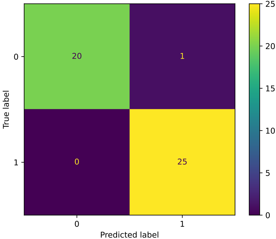
Confusion Matrix for Tuned CatBoost Model
